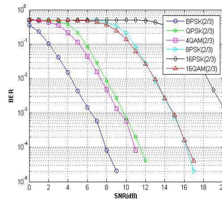
Figure 3. BER simulations of an audio data through WiMAX PHY layer using \frac{2}{3} -rated Convolutionally encoded system for different modulation schemes over an AWGN channel.
