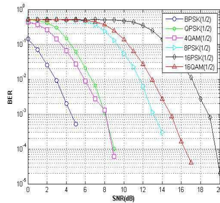
Figure 2 BER simulations of an audio data through WiMAX-PHY layer using \frac{1}{2} -rated Convolutionally encoded system for different modulation schemes over an AWGN channel
